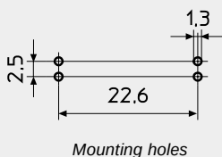
Mounting holes
