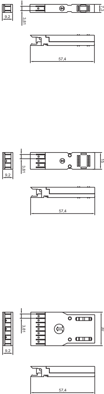
1 Pair 110 Patch Plug 2 Pairs 110 Patch Plug 4 Pairs 110 Patch Plug
