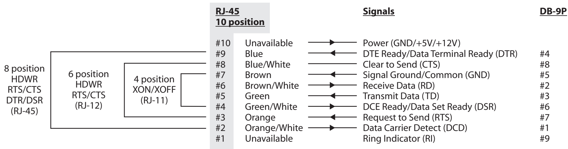
RJ-45
