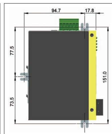
Panel Dimension
