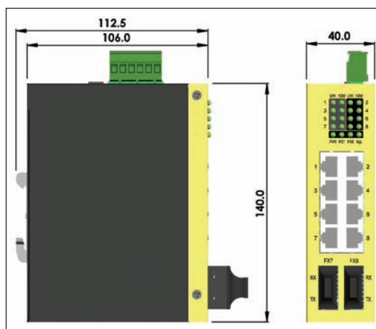
DIN-Rail Dimension
