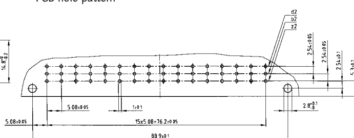
PCB-hole pattern
