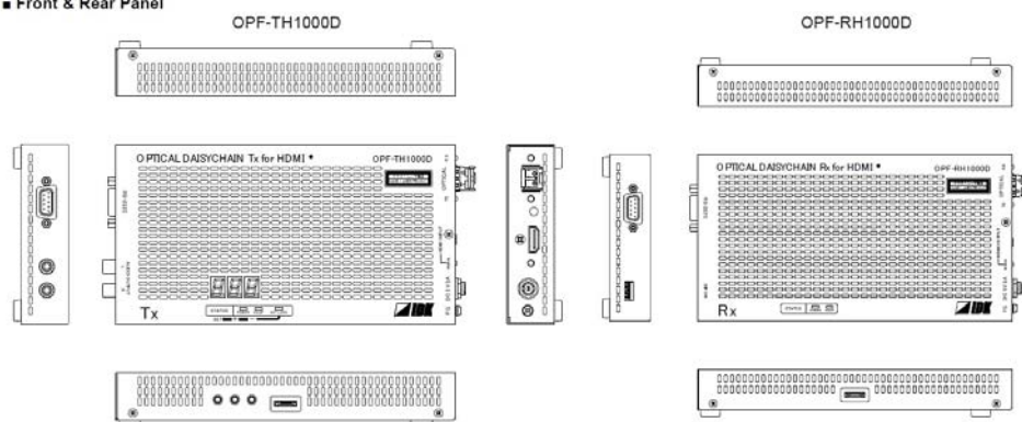
■ Front & Rear Panel
