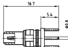
Plug contact
