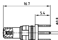
Plug contact
