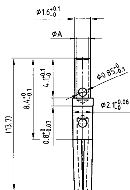
gedreht screw machined version
