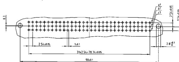
PCB-hole pattern
