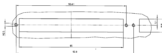
Panel cutout
