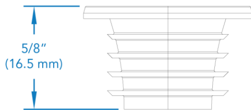
HPG-10 (Side View)
