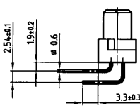
Solder pin angled
