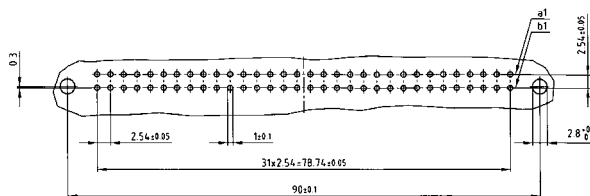
PCB-hole pattern
