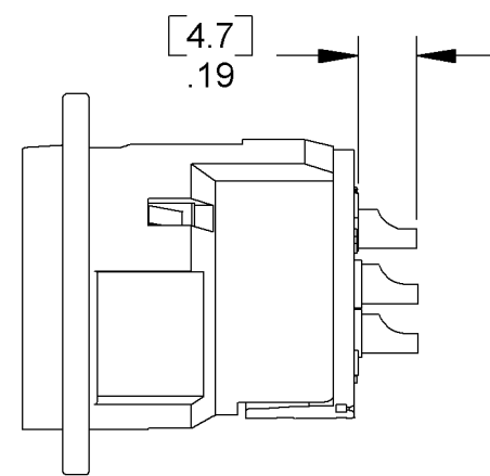
MALE SOLDER CUP OPTION "SC"
