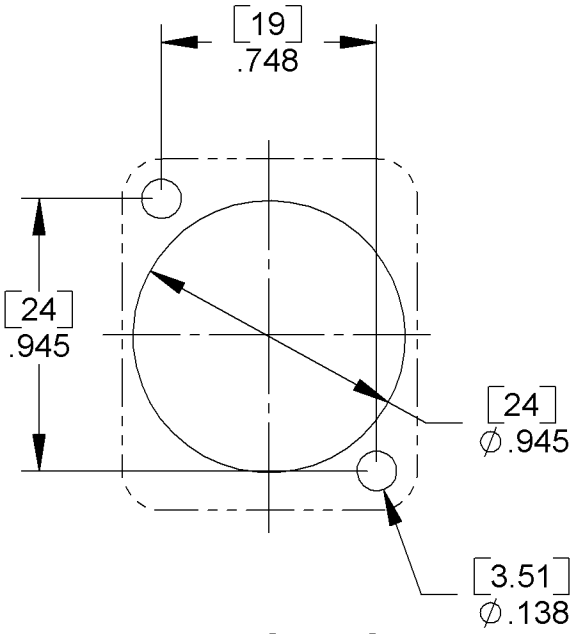
PANEL CUT-OUT FRONT OR REAR MOUNT
