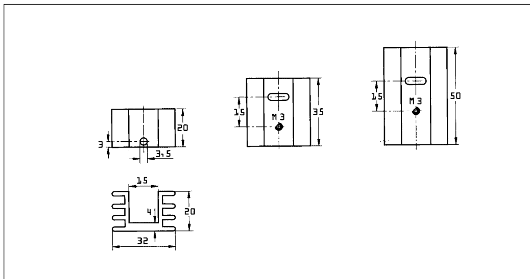
TO 126 (SOT 32)
