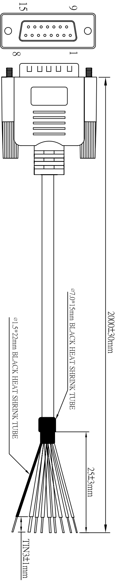
DB 15M(NICKEL PLATED) BEIGE MOLDING
