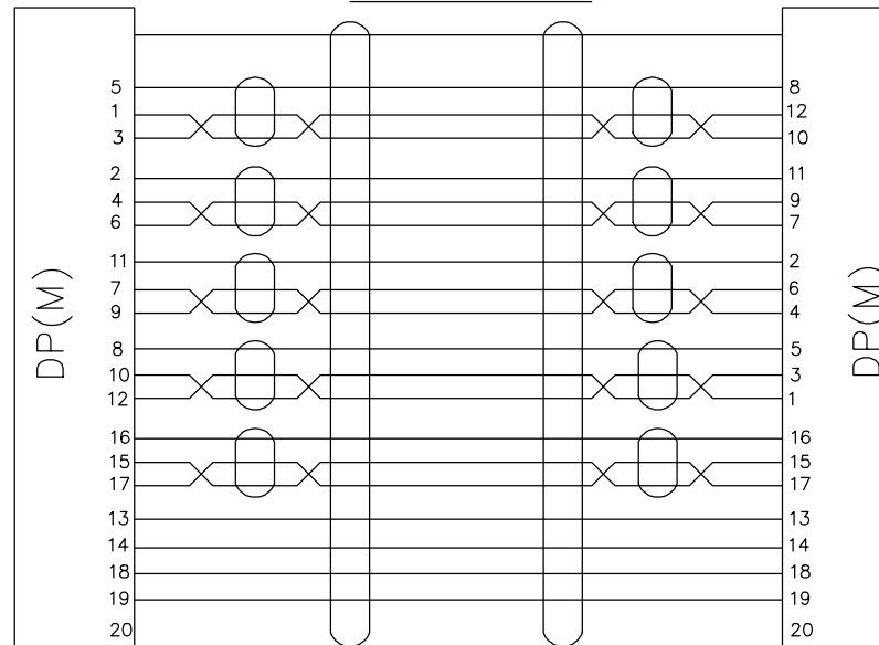
Signal Assignment
