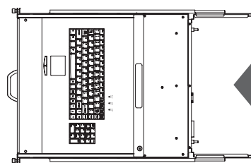
Console body
