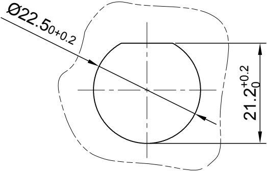
MOUNTING HOLE
