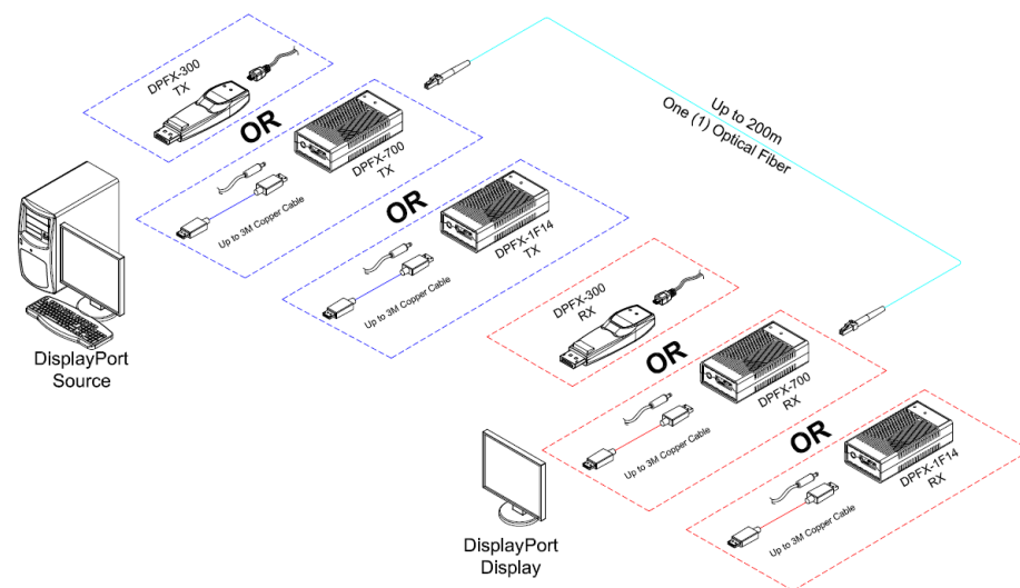
Fig Figure 3 – Connection of optical fiber
