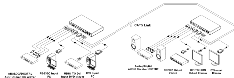
Figure 1 – Overall Digital Video/Audio and Serial I/O Extender
