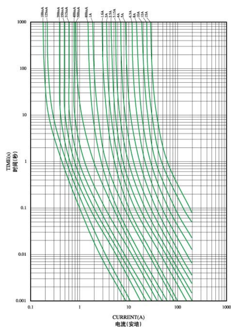
50T RoHS I-T CHARACTERISTICS CURVE 50T RoHS 电流-时间曲线图
