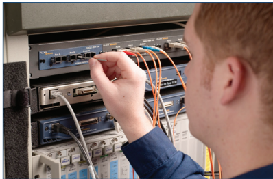
Insert the swab into the port and turn several times while applying gentle pressure. Follow the damp swab with a dry one, using the same procedure to remove any remaining solvent from the end-face and alignment sleeve.
