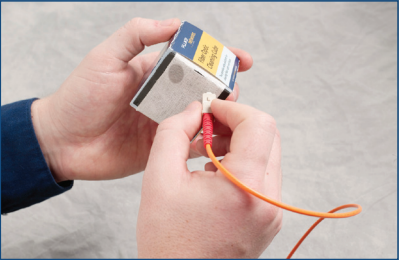
Holding the connector perpendicularly, swipe the end-face from the wet spot into a dry zone.
