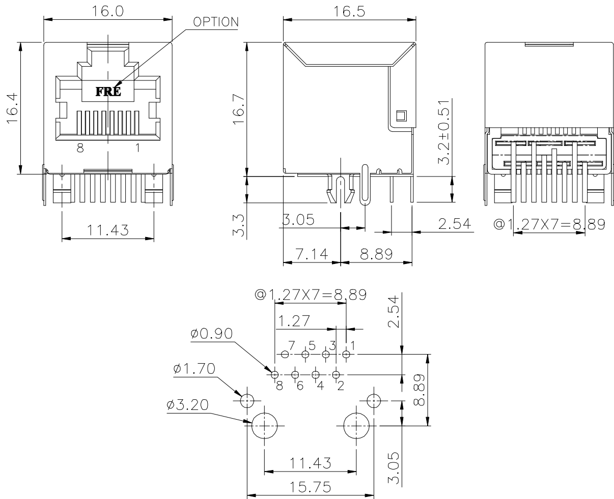
PC BOARD LAYOUT t=1.60mm COMPONENT SIDE SHOWN
