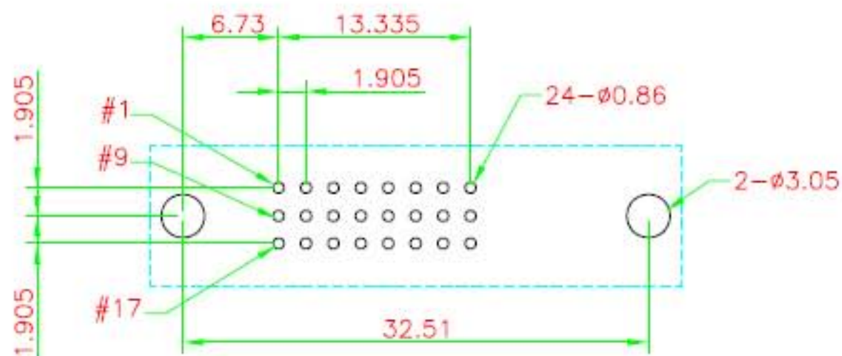
PCB LAYOUT
