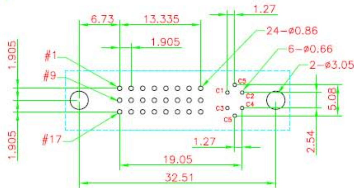
PCB LAYOUT
