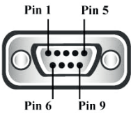
RS232 Pinout (9 Pin Male)
