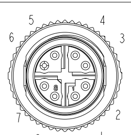
Conn.1&2 Pin Assignment Front View
