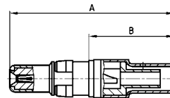
Plug contact
