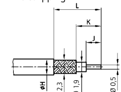
Wire stripping
