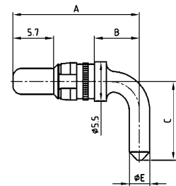
Premating contact
