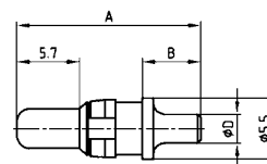
Plug contact
