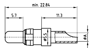
Plug contact
