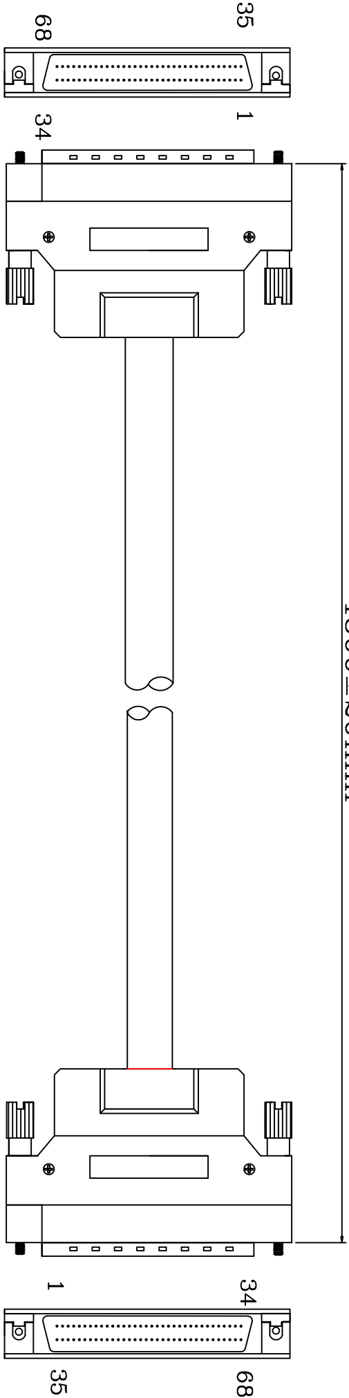
HPD68M Assembly Metal shell
