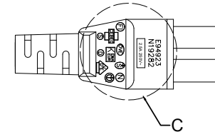
IEC60320 C5 (SF-87)
