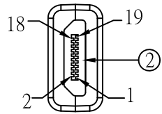
HDMI 19F(Nickel plated)
