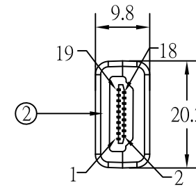
HDMI 19F(Nickel plated)
