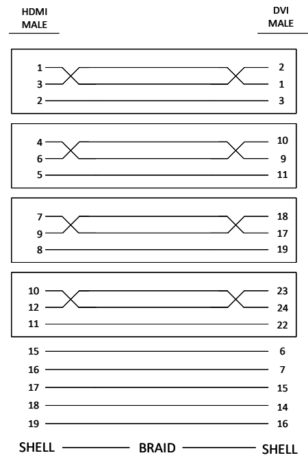
PINOUT CONFIGURATION
