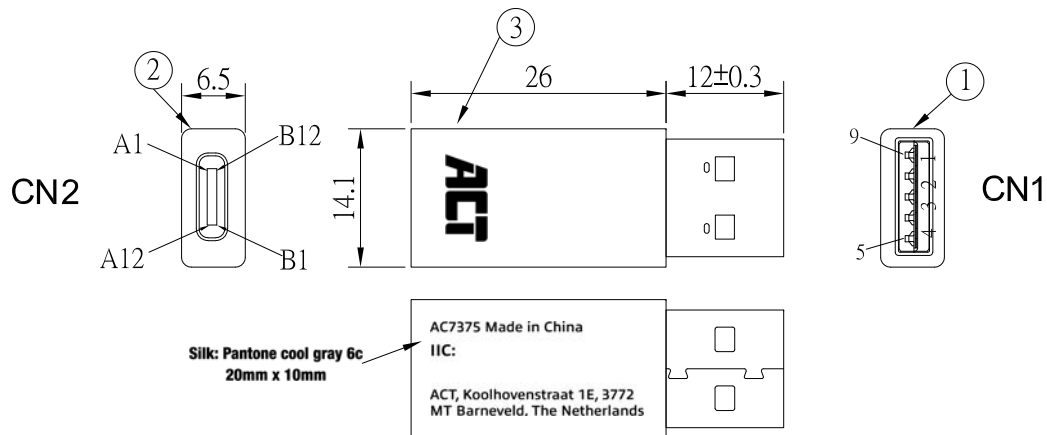
USB3.0 AM-Type CF Adapter Silver Metal Assembly Shell TOL:±0.5mm
